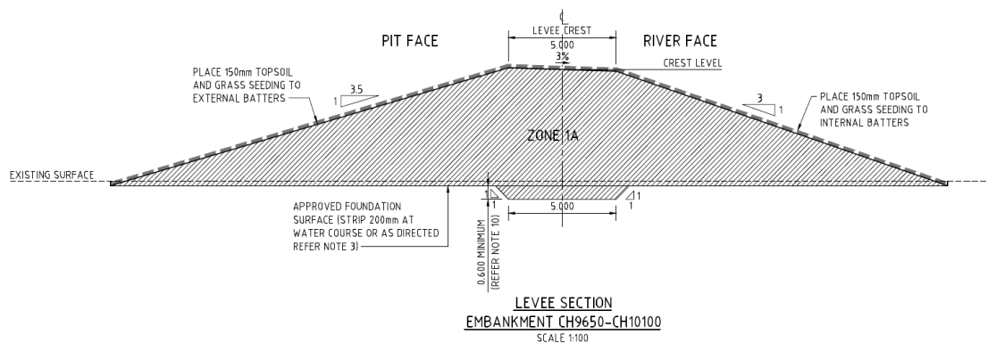
Figure 9.4: Conceptual levee cross-section
