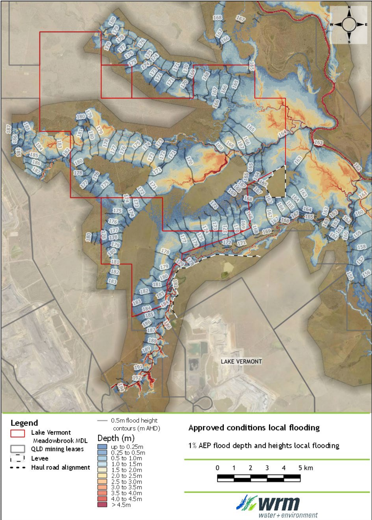
Figure 9.8: 1% AEP approved conditions local flood depths and heights
