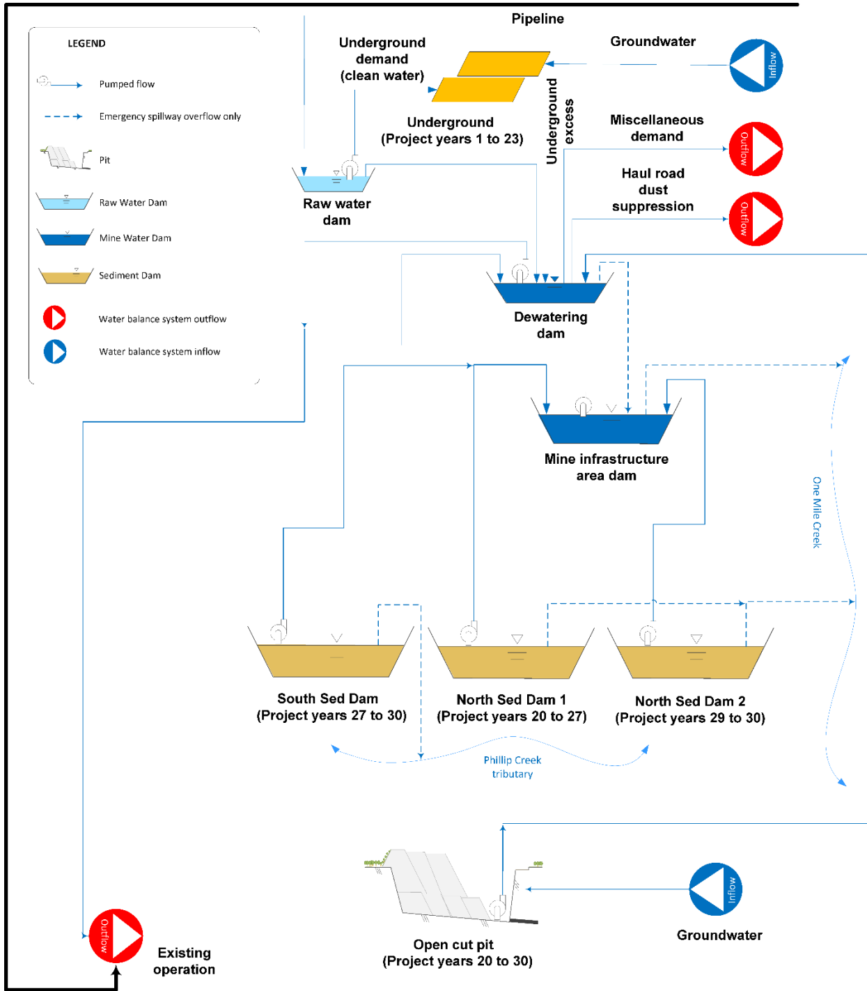
Figure 8.8: Water management system schematic
