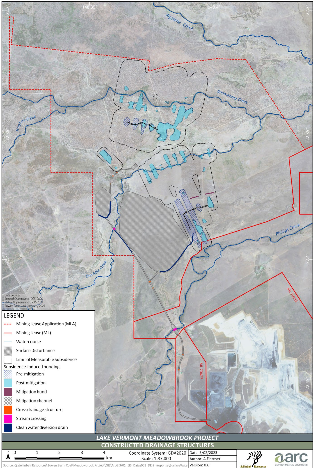
Figure 8.6: Indicative cross drainage and flow diversion drains.
