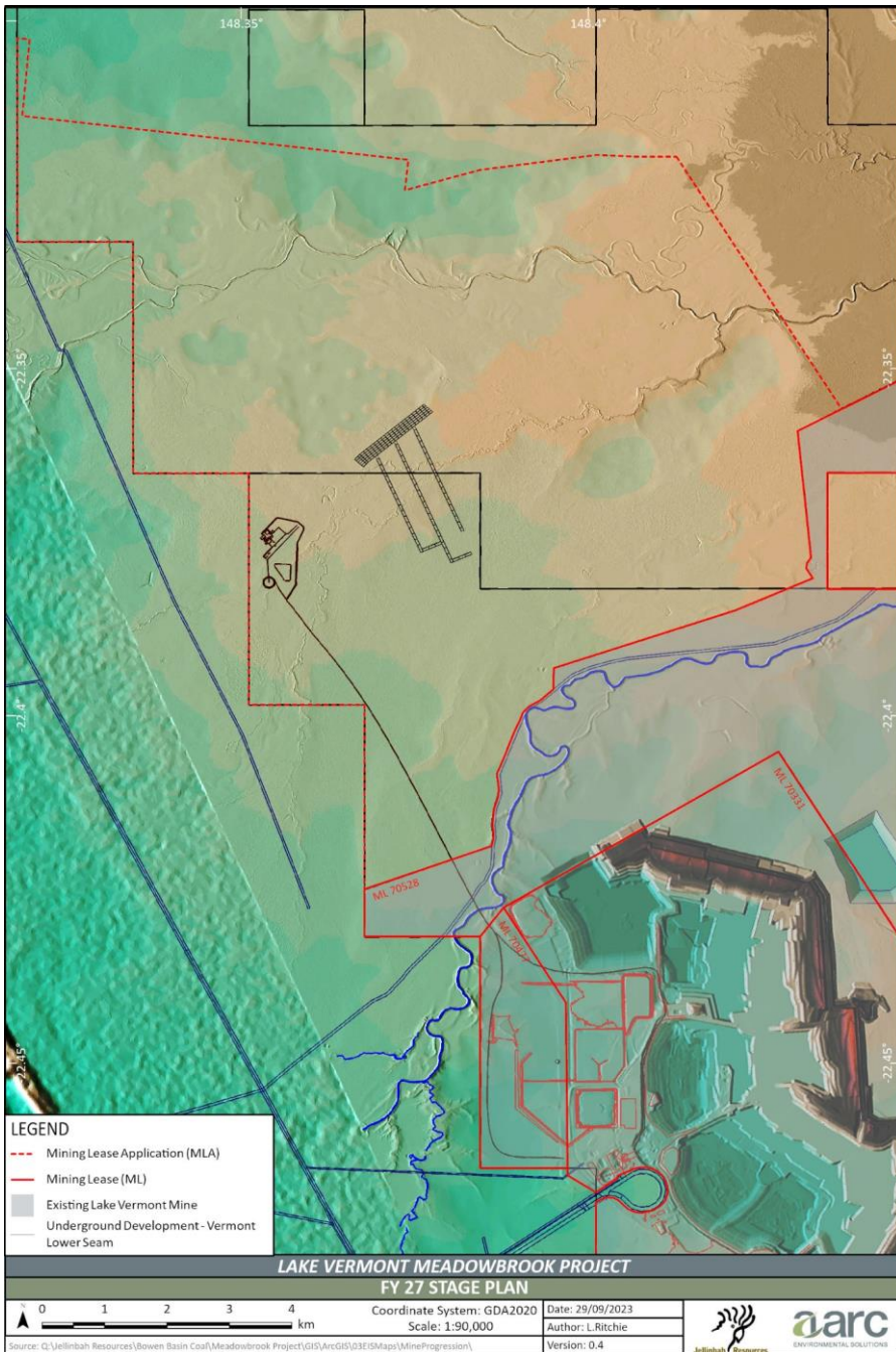
Figure 3.29: Mine stage plan—Project Year 2
