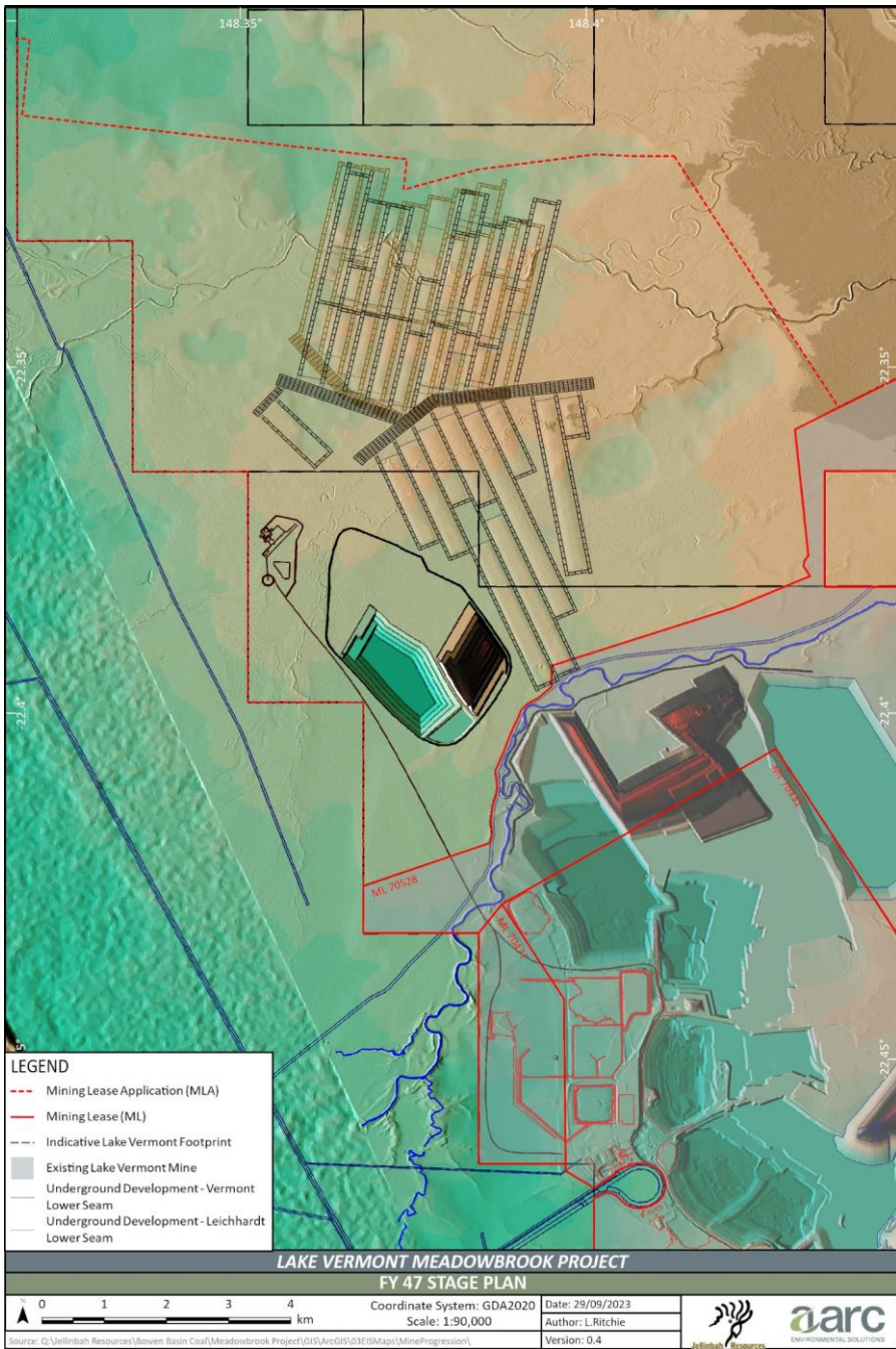
Figure 3.33: Mine stage plan—Project Year 22
