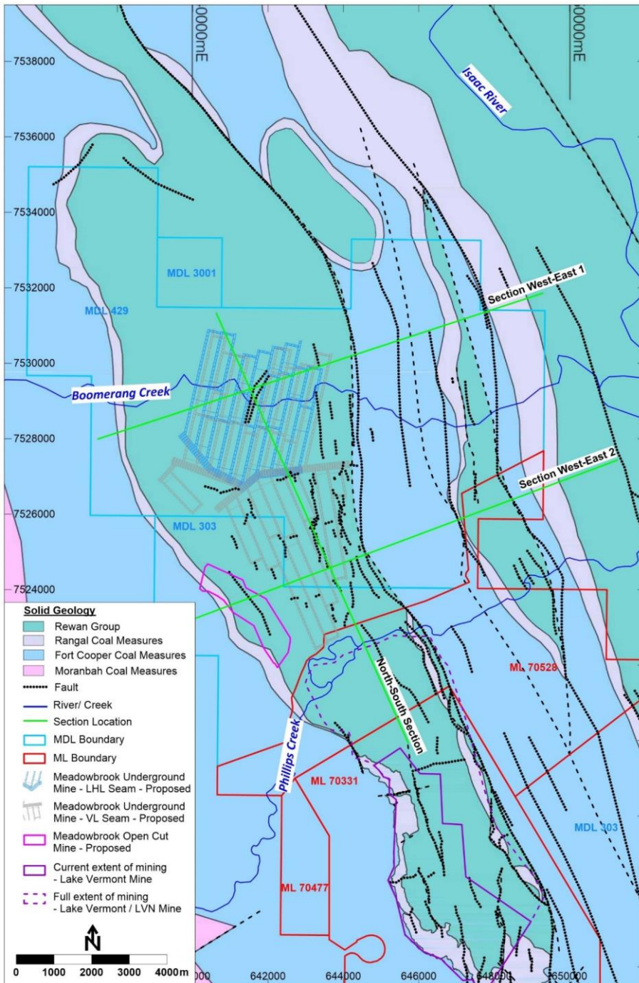
Figure 3.15: Geology of the Project site
