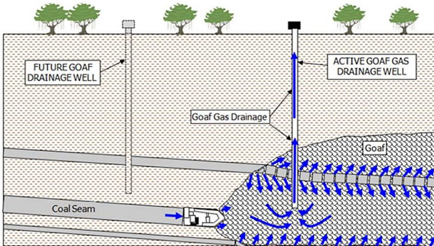
Figure 3.41: Vertical goaf gas wells—example installation.
