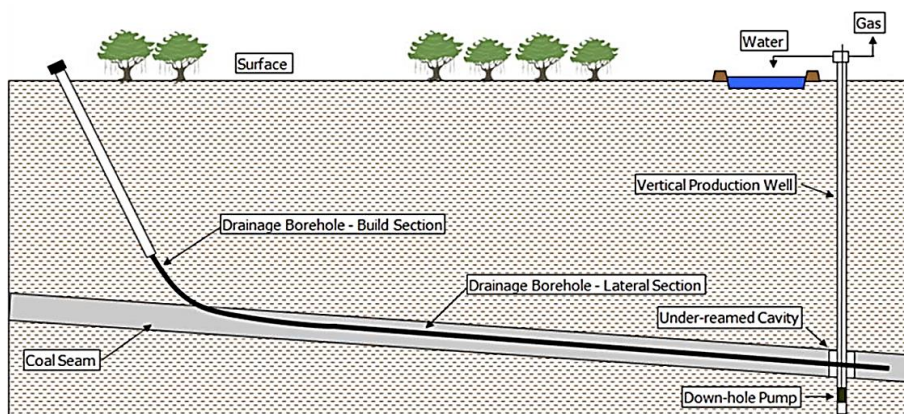
Figure 3.37: SIS Gas Drainage Underground Installation Example.
