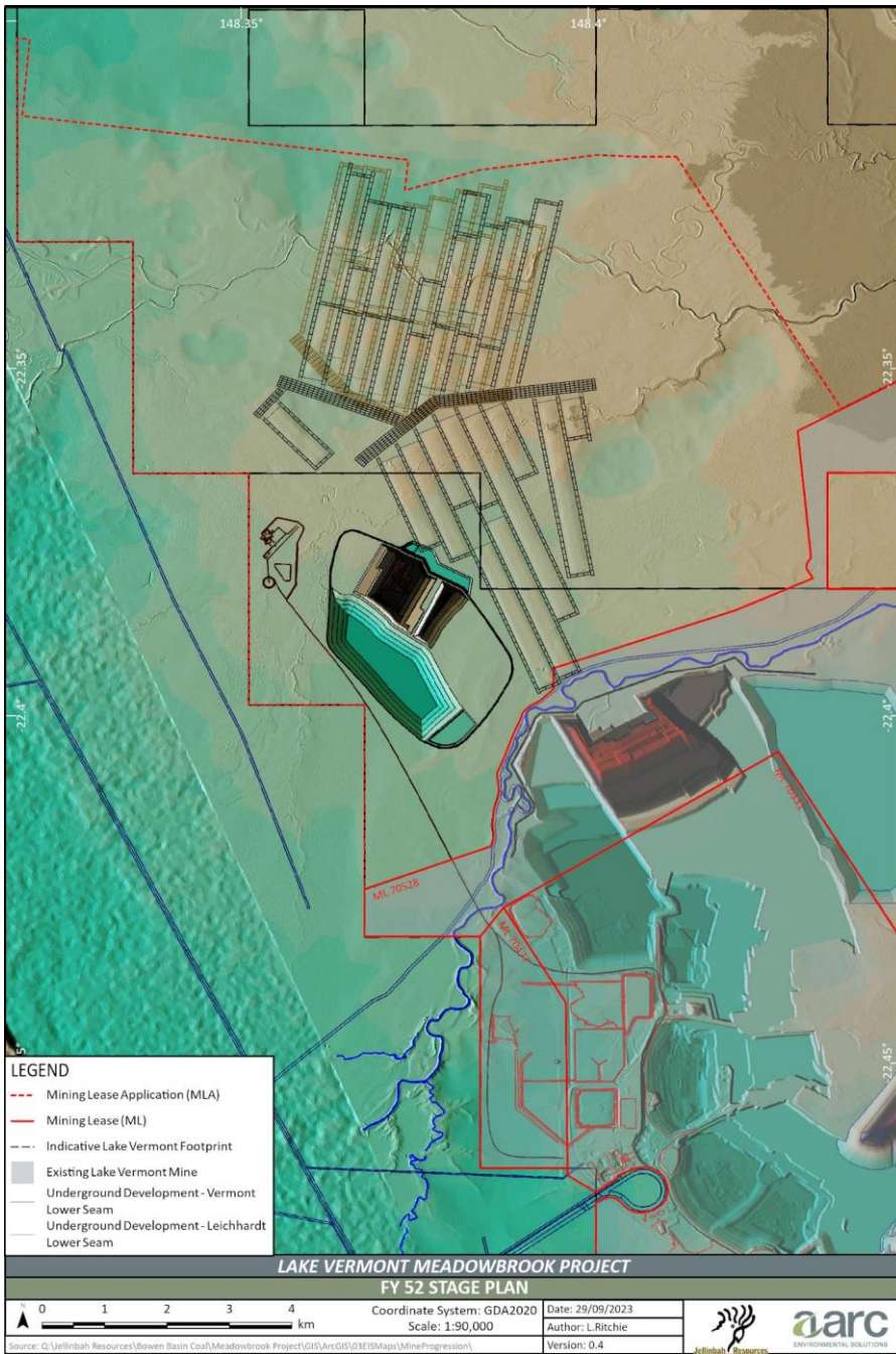
Figure 3.34: Mine stage plan—Project Year 27
