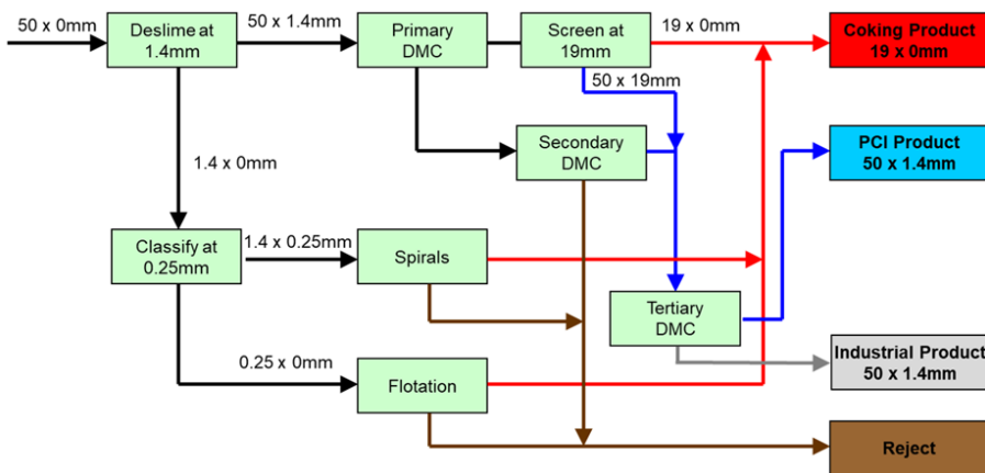
Figure 3.43: CHPP module schematic
