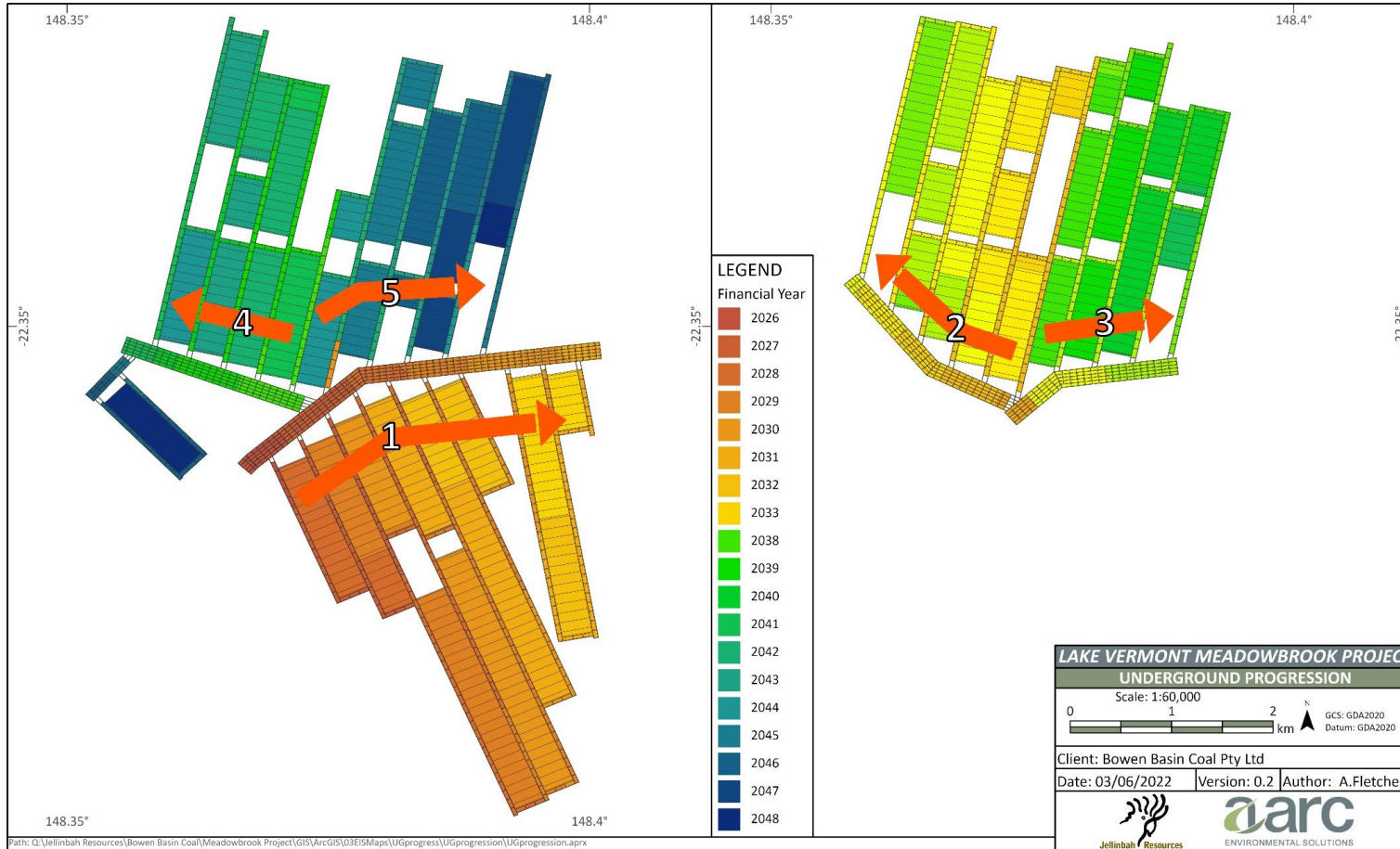
Figure 3.26: Indicative mine progression plans—underground mining
