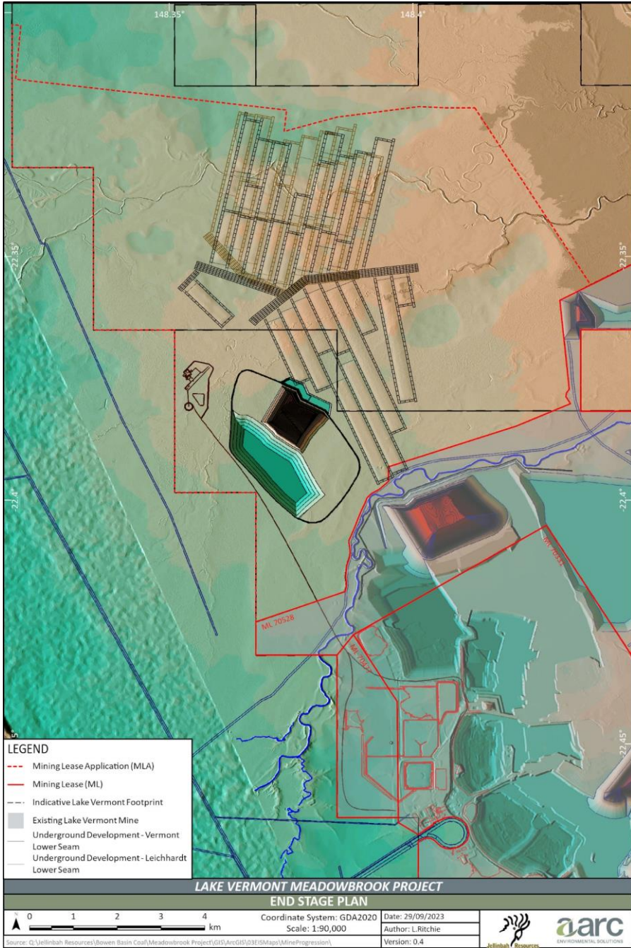
Figure 3.35: Mine stage plan—end of all mining
