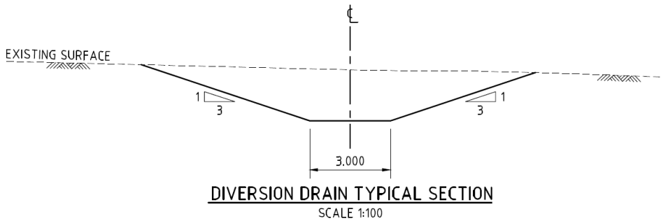
Figure 3.25: Conceptual diversion drain cross-section
