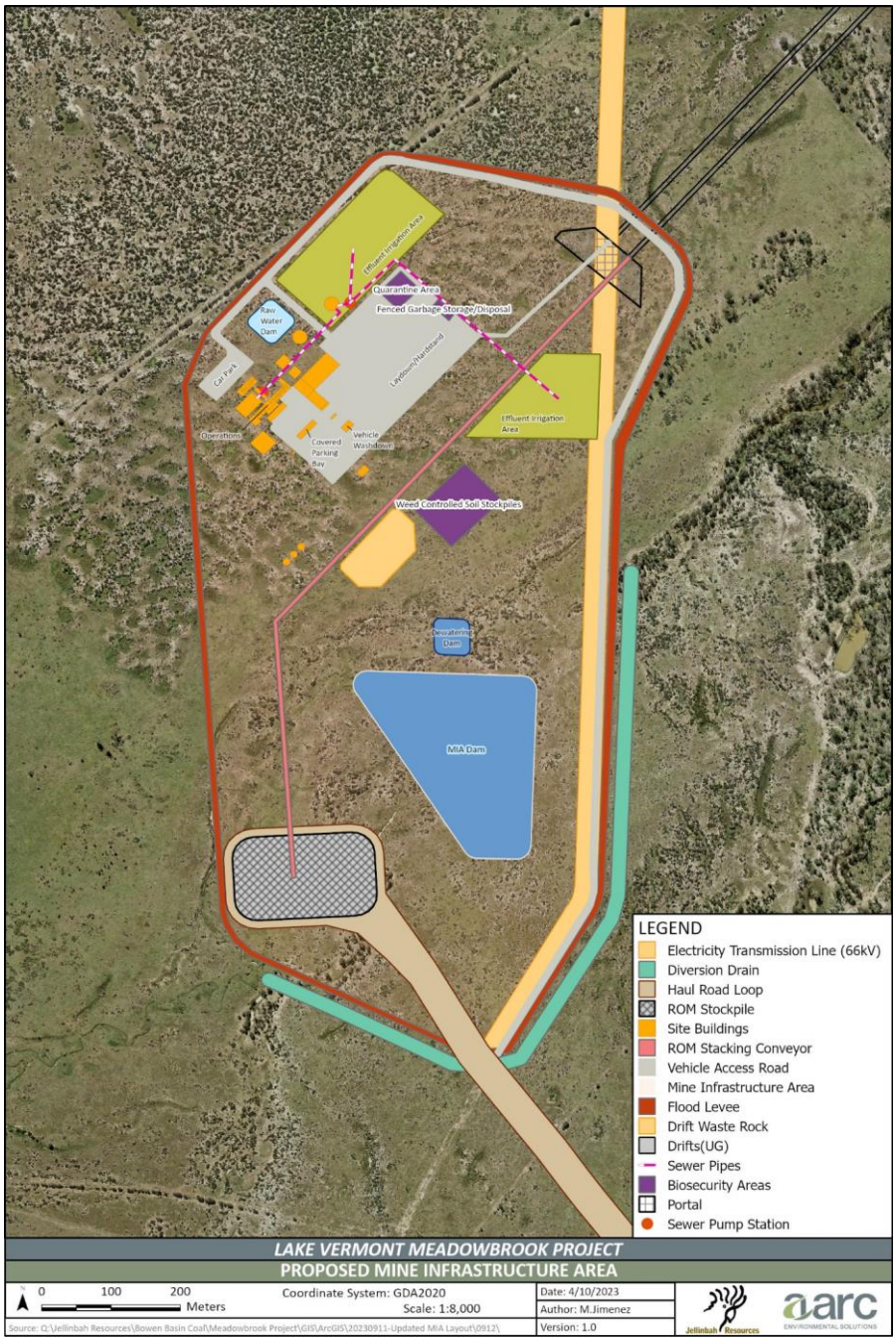
Figure 3.24: Proposed layout of the mine infrastructure area
