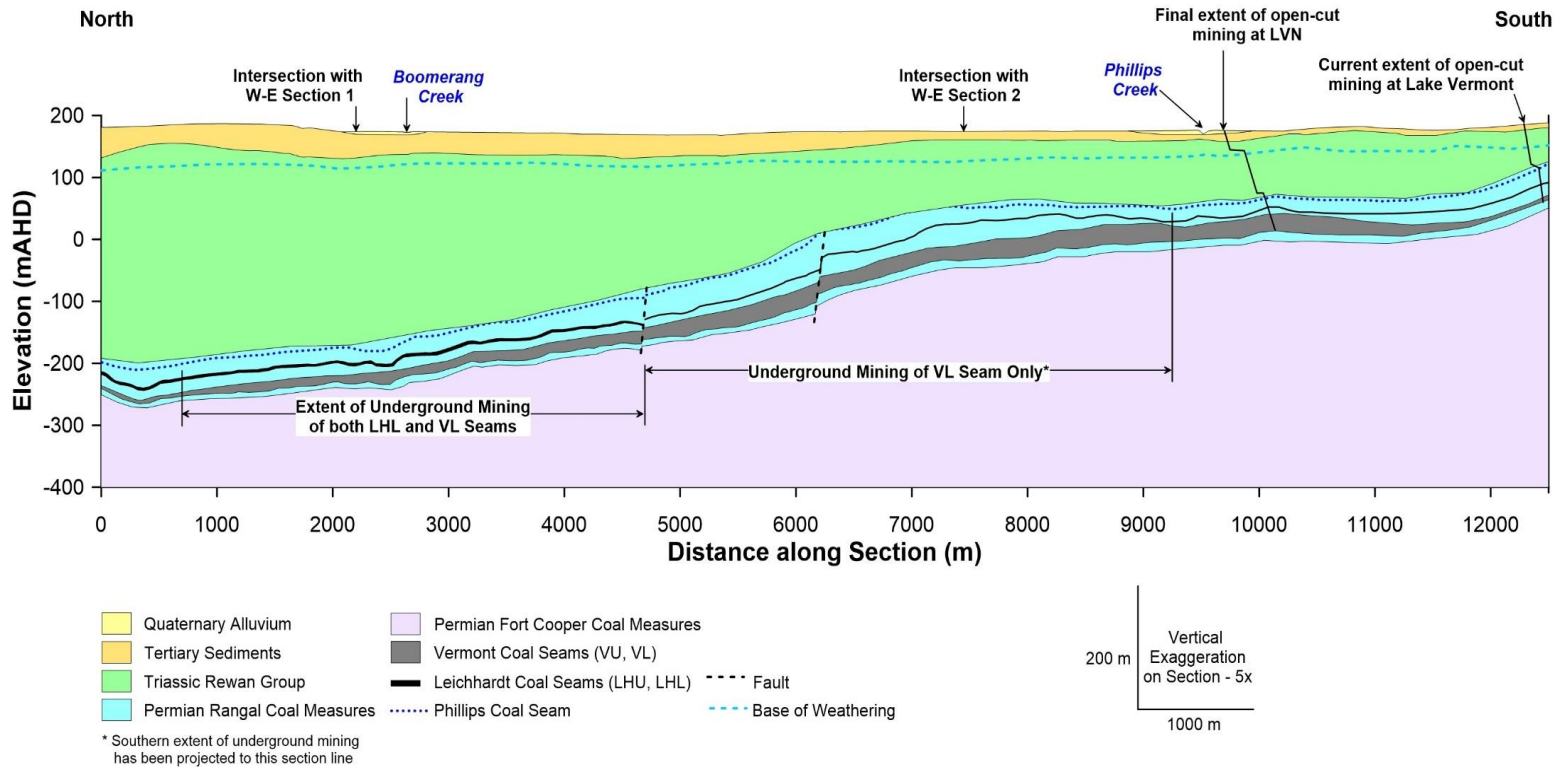
Figure 3.18: North-south cross-section of Project geology
