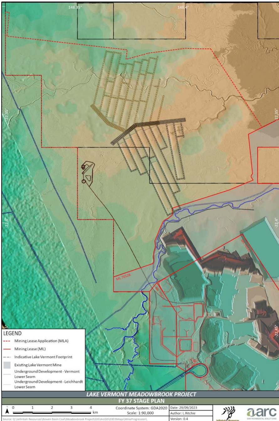
Figure 3.31: Mine stage plan—Project Year 12
