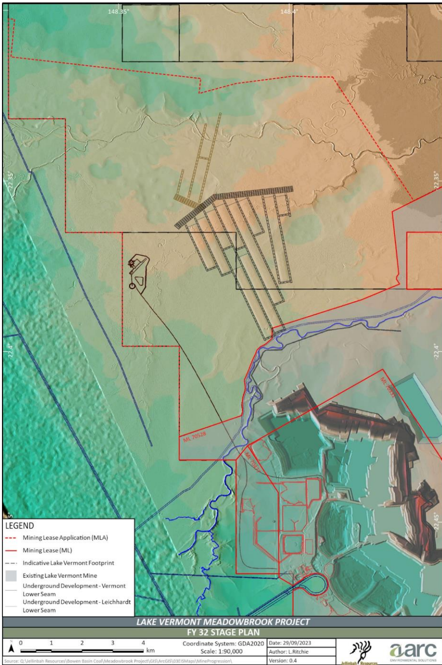
Figure 3.30: Mine stage plan—Project Year 7
