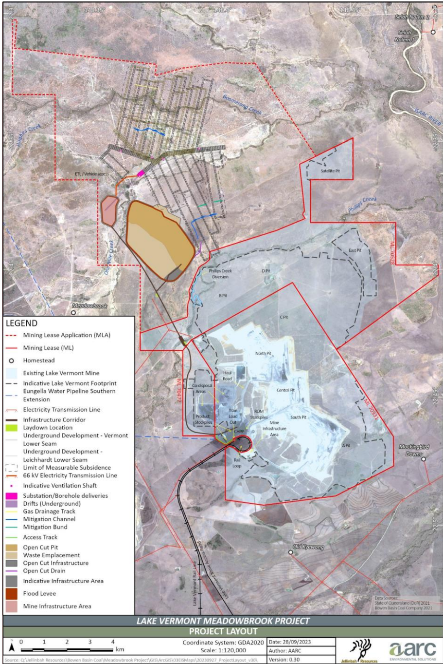
Figure 3.2: Project layout
