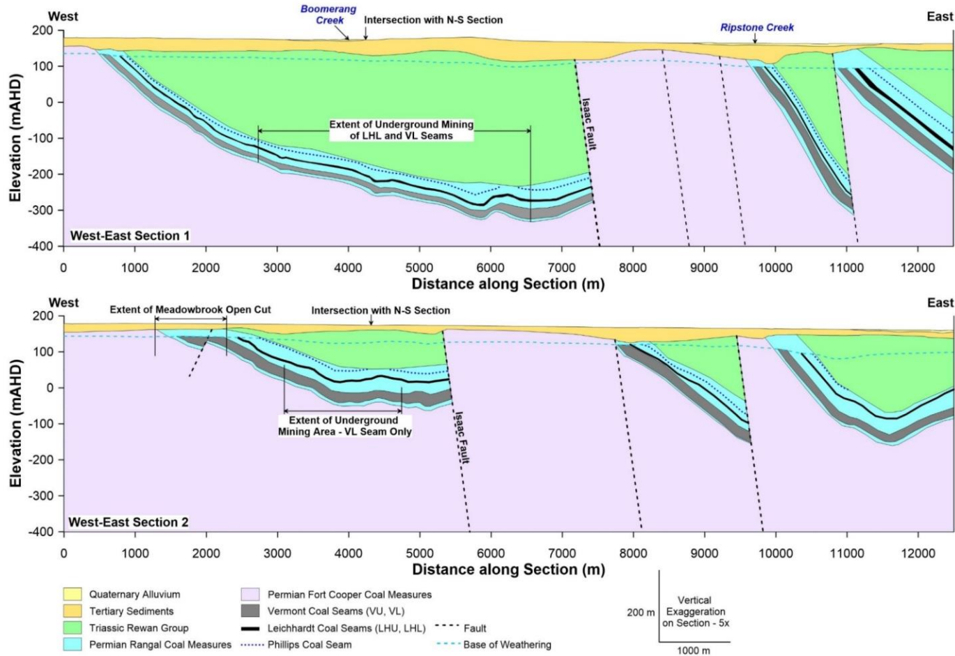
Figure 3.17: West-east cross-sections of Project geology
