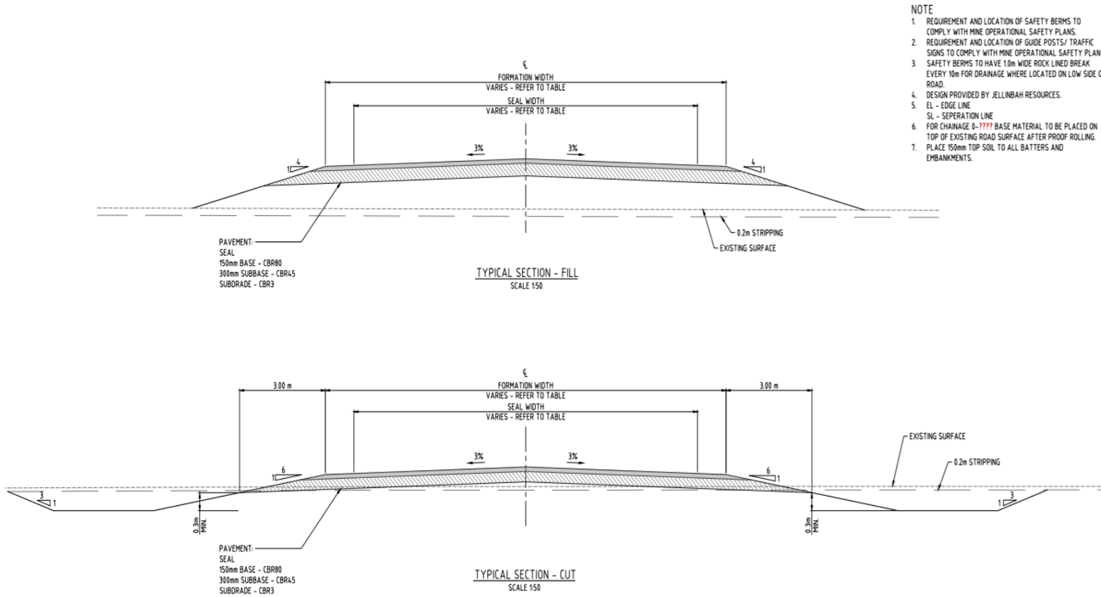
Figure 3.22: Conceptual cross-sections of the Project access/haulage road
