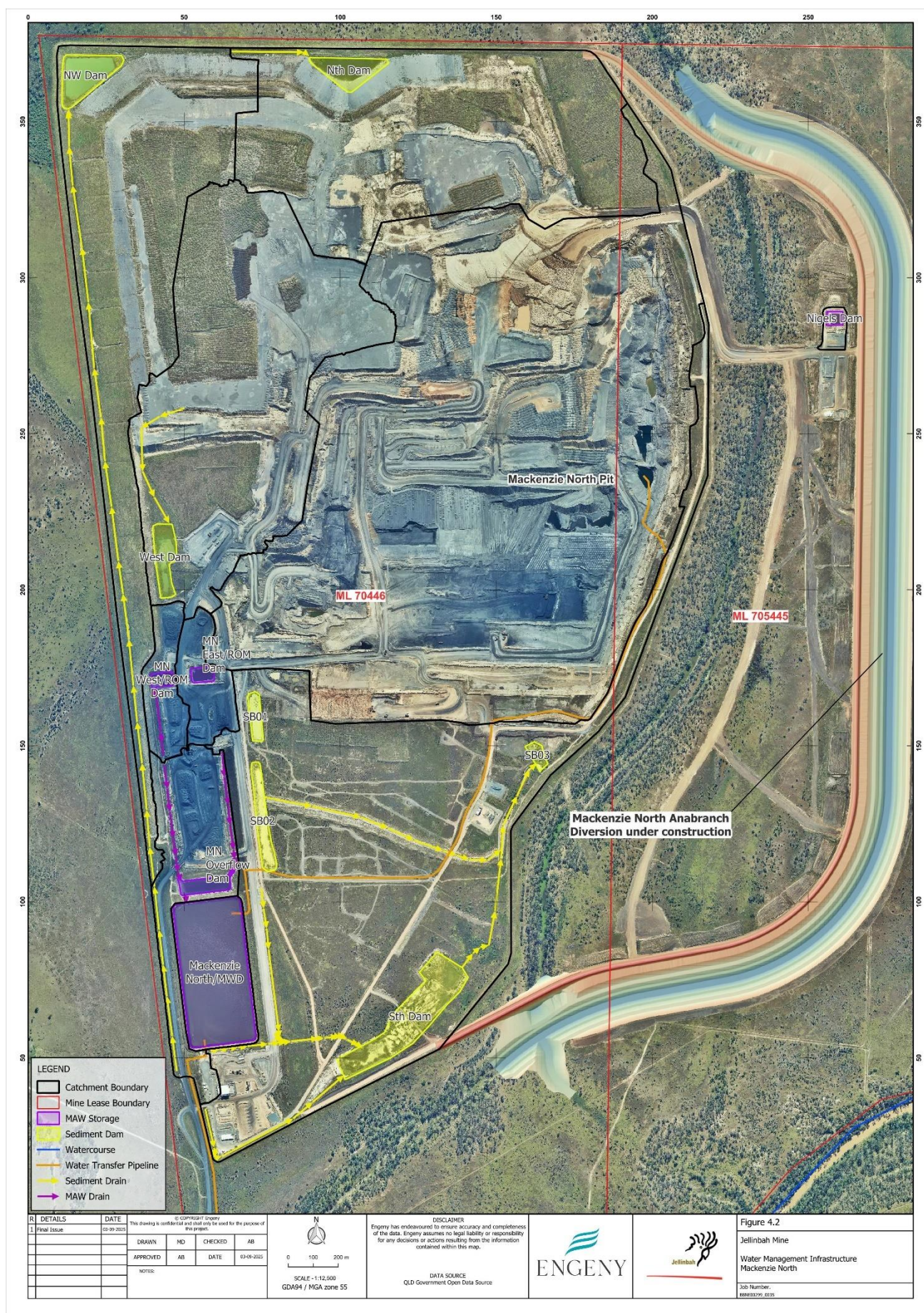
Figure 4.2: Water Management Infrastructure – Mackenzie North WATER MANAGEMENT PLAN | BBNE00299_0034-REP-002-0
