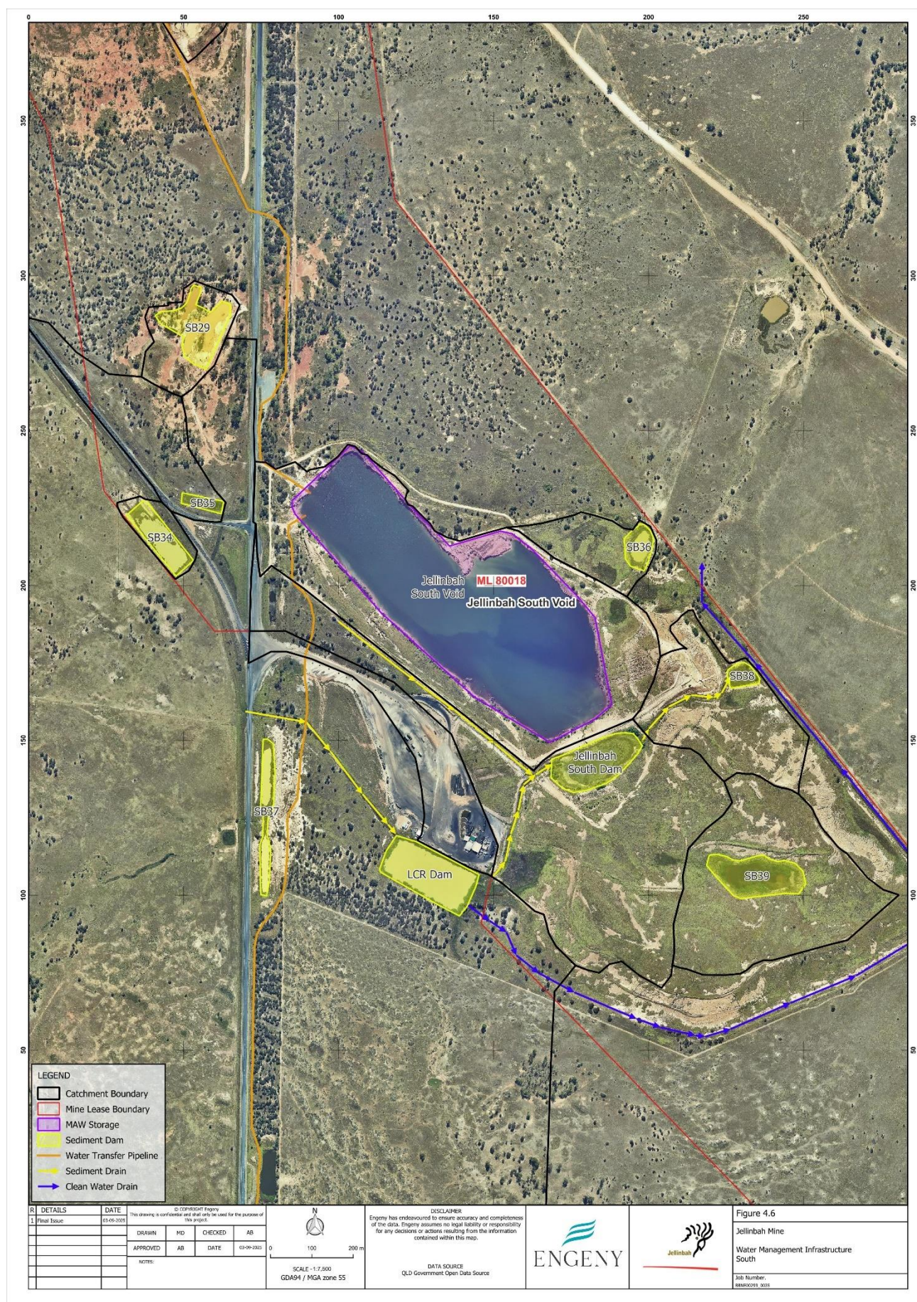
Figure 4.6: Water Management Infrastructure – South
