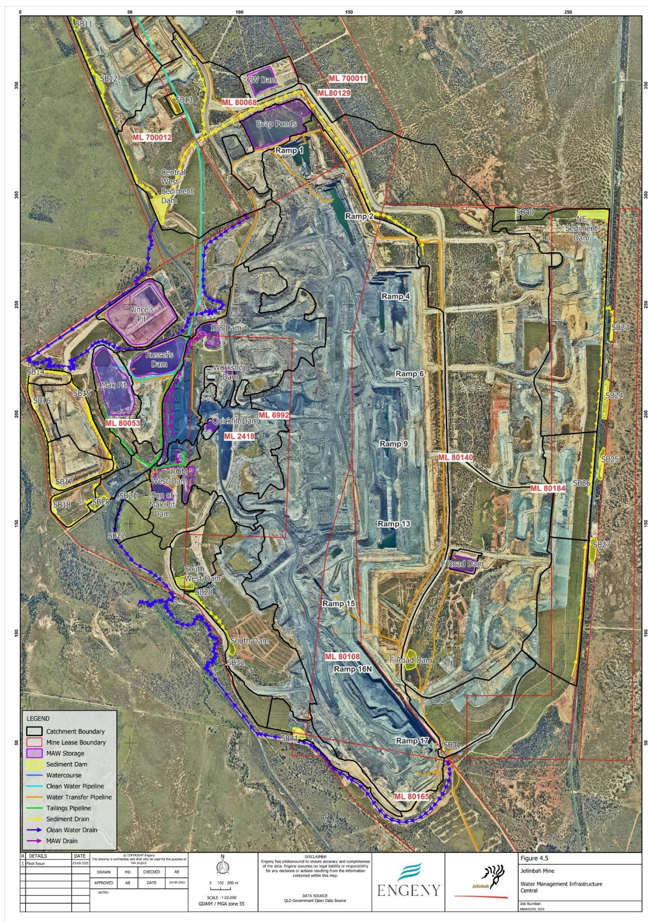
Figure 4.5: Water Management Infrastructure – Central WATER MANAGEMENT PLAN | BBNE00299_0034-REP-002-0
