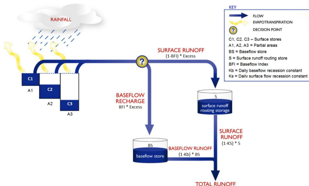
Figure 5.2: AWBM Schematic
