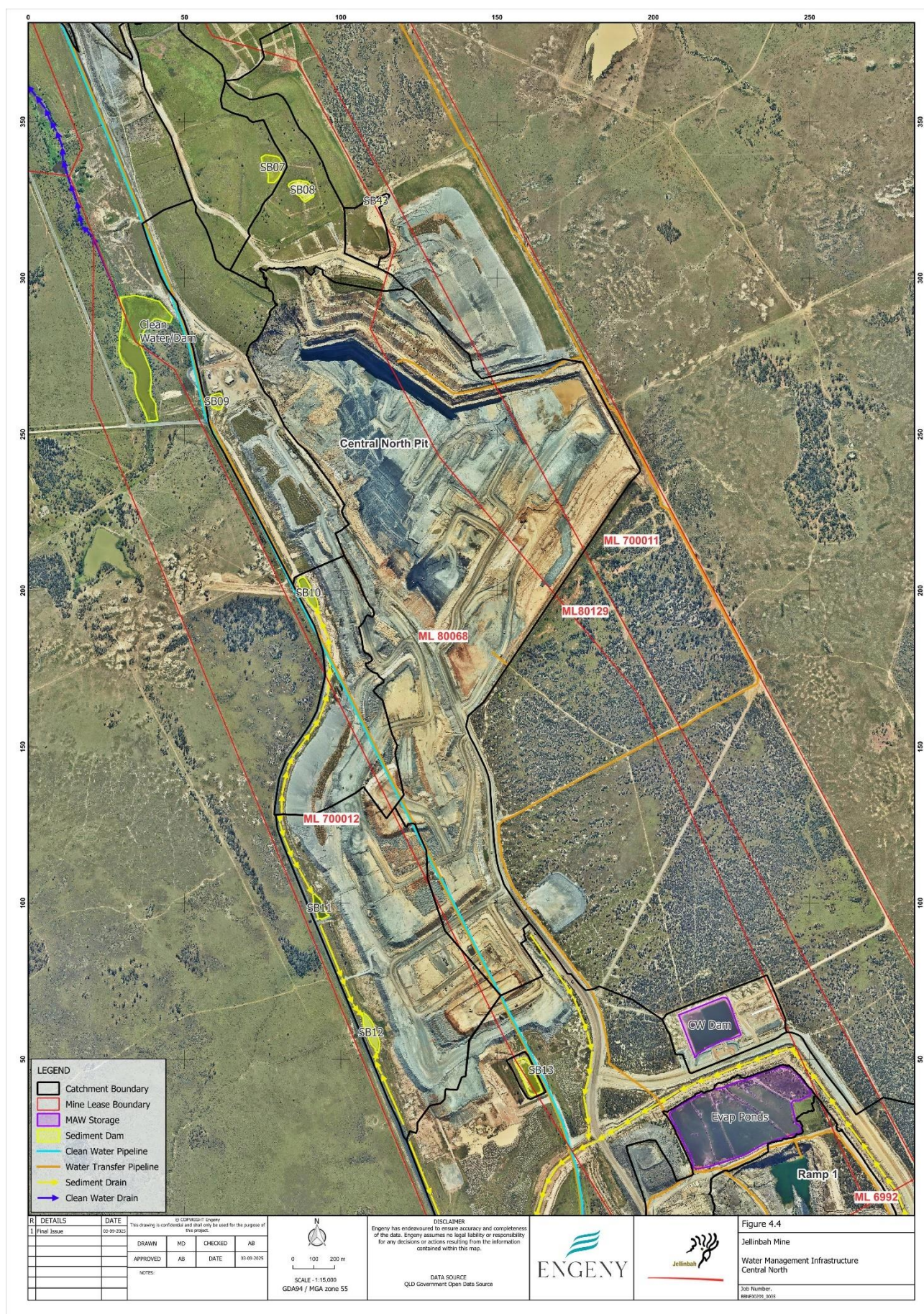
Figure 4.4: Water Management Infrastructure – Central North
