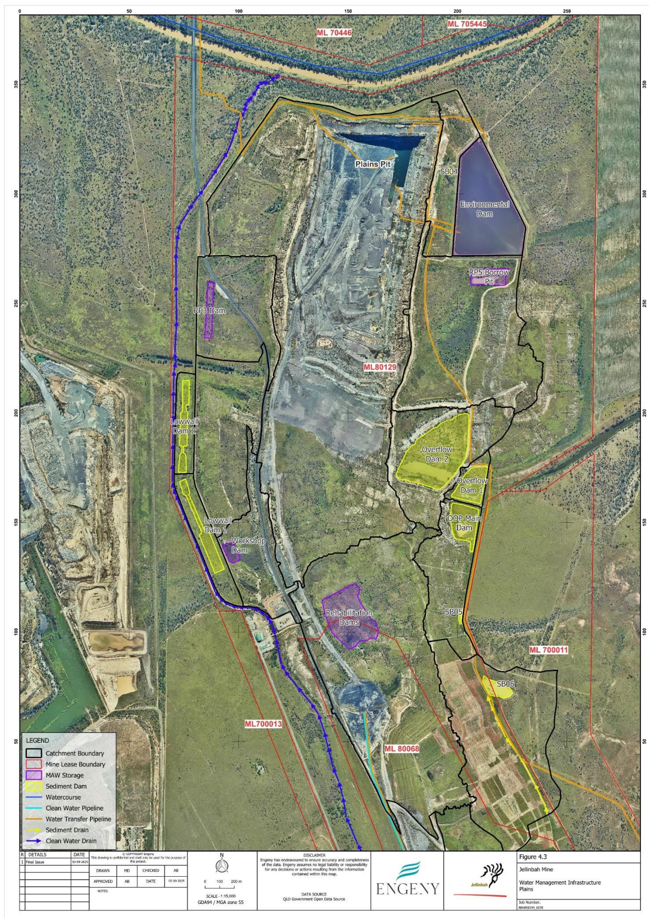
Figure 4.3: Water Management Infrastructure – Plains
