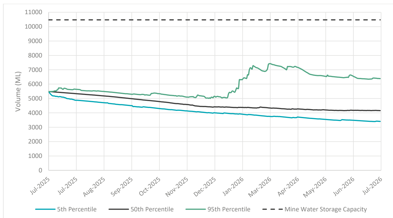
Figure 5.6: Mine Water System Inventory Forecast Result
