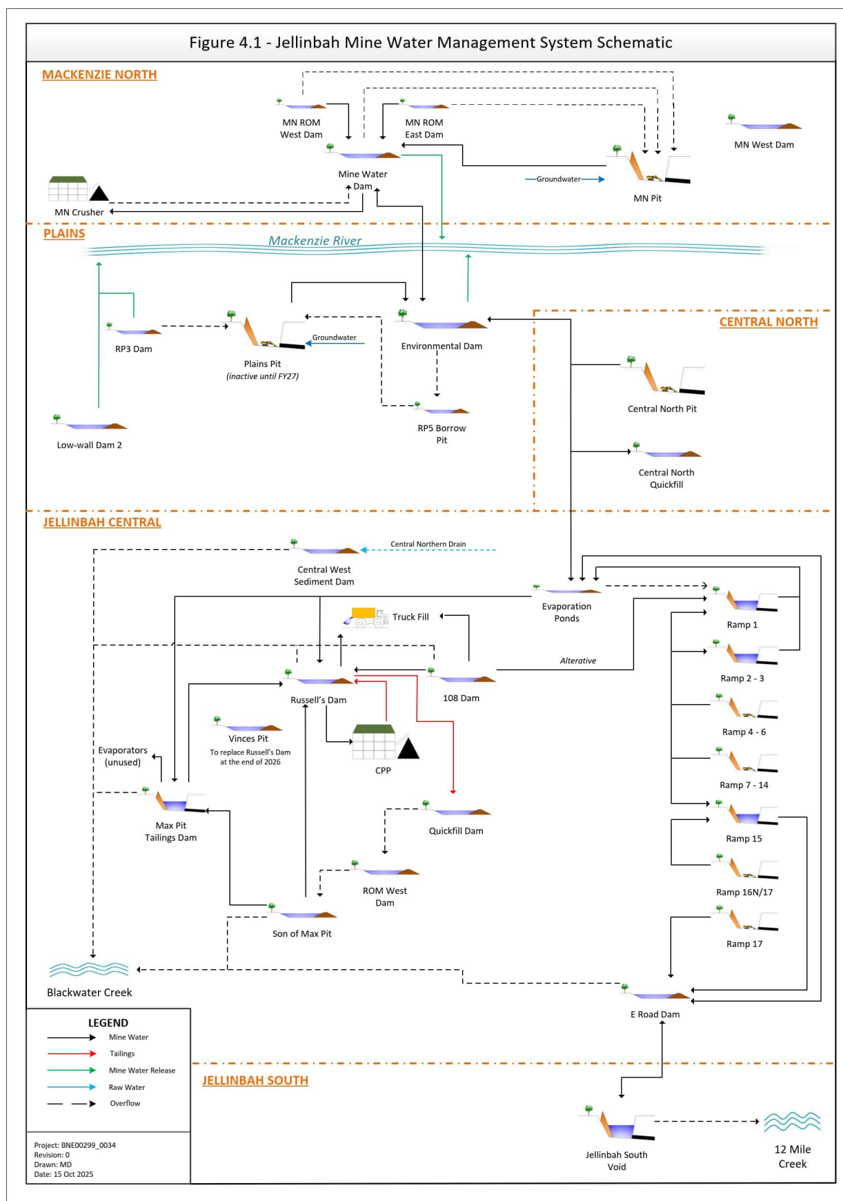
Figure 4.1: Water Management System Schematic
