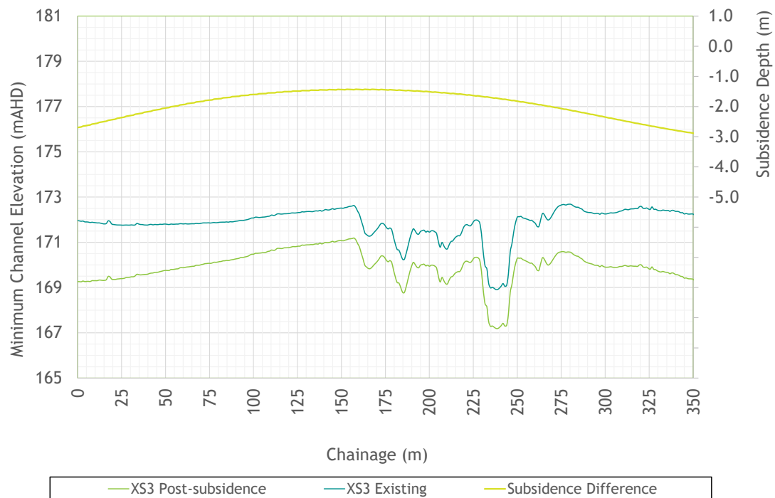
Figure 3.25 - Cross-section - Boomerang Creek main channel Ch 13,220
