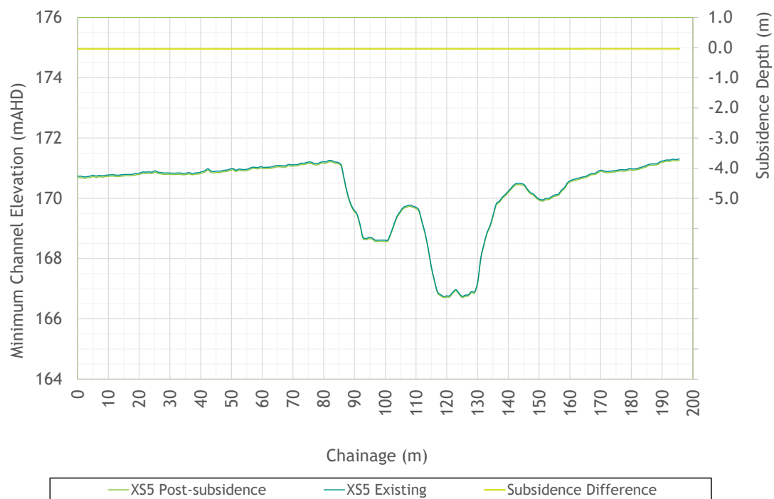
Figure 3.27 - Cross-section - Boomerang Creek main channel Ch 14,620
