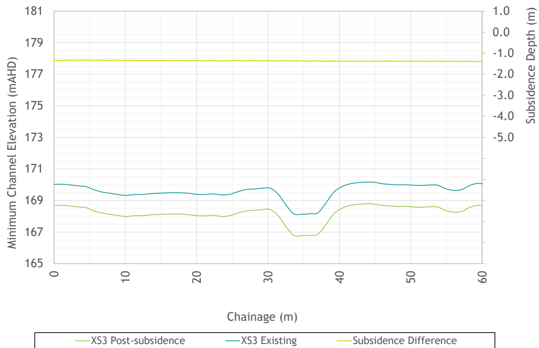
Figure 3.33 - Cross-sections - One Mile Creek main channel Ch 11,830
