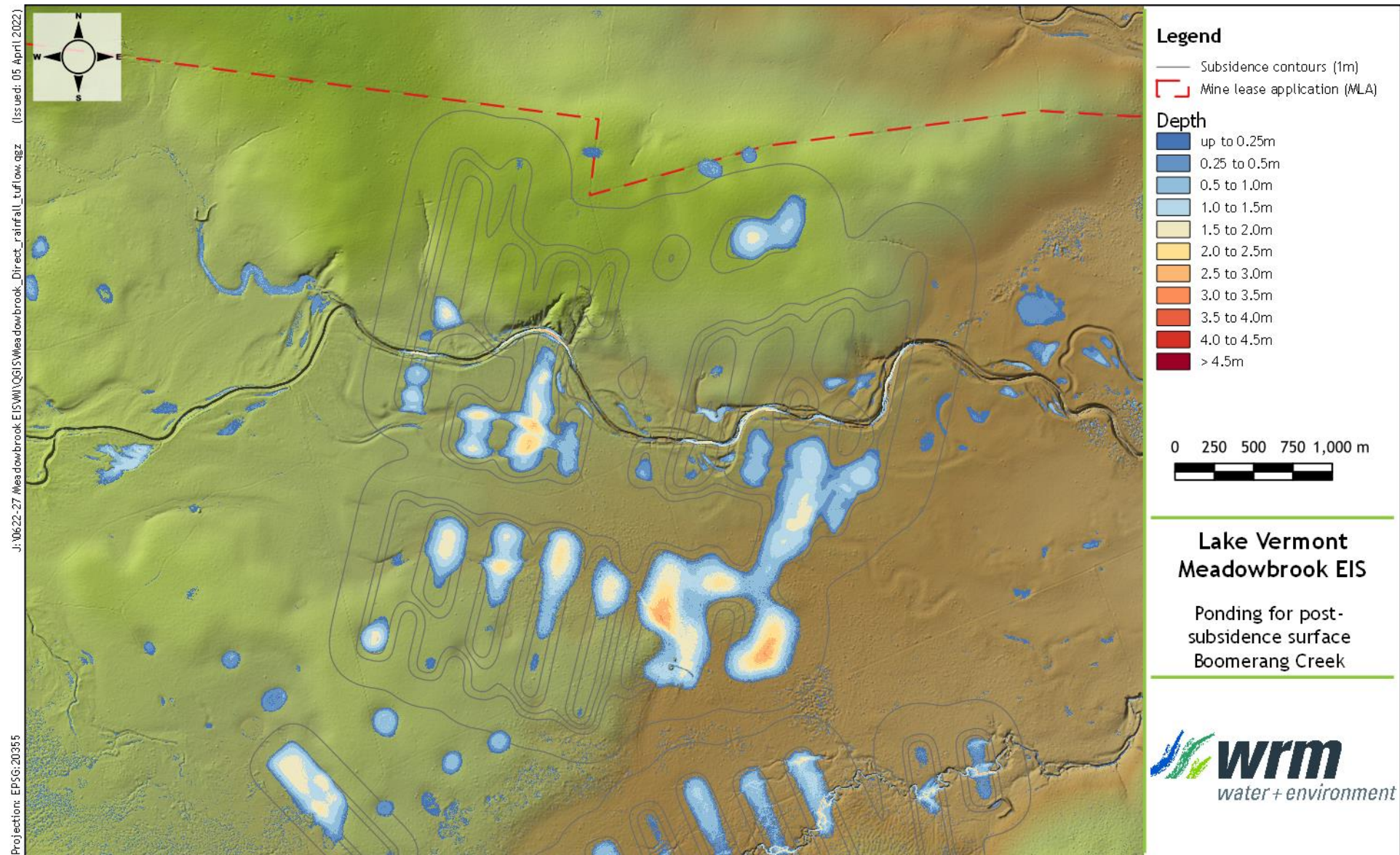
Figure 3.14 - Post-subsidence ponding (Boomerang Creek)
