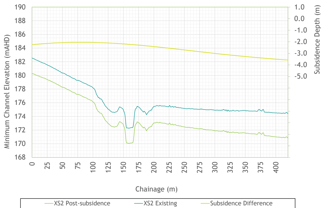
Figure 3.24 - Cross-section - Boomerang Creek main channel Ch 10,590
