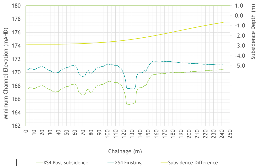
Figure 3.26 - Cross-section - Boomerang Creek main channel Ch 14,170
