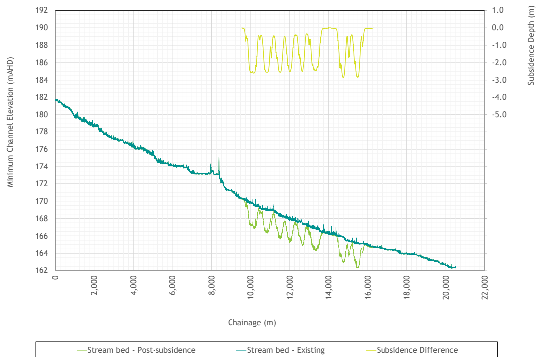
Figure 3.29 - Longitudinal profile - One Mile Creek main channel
