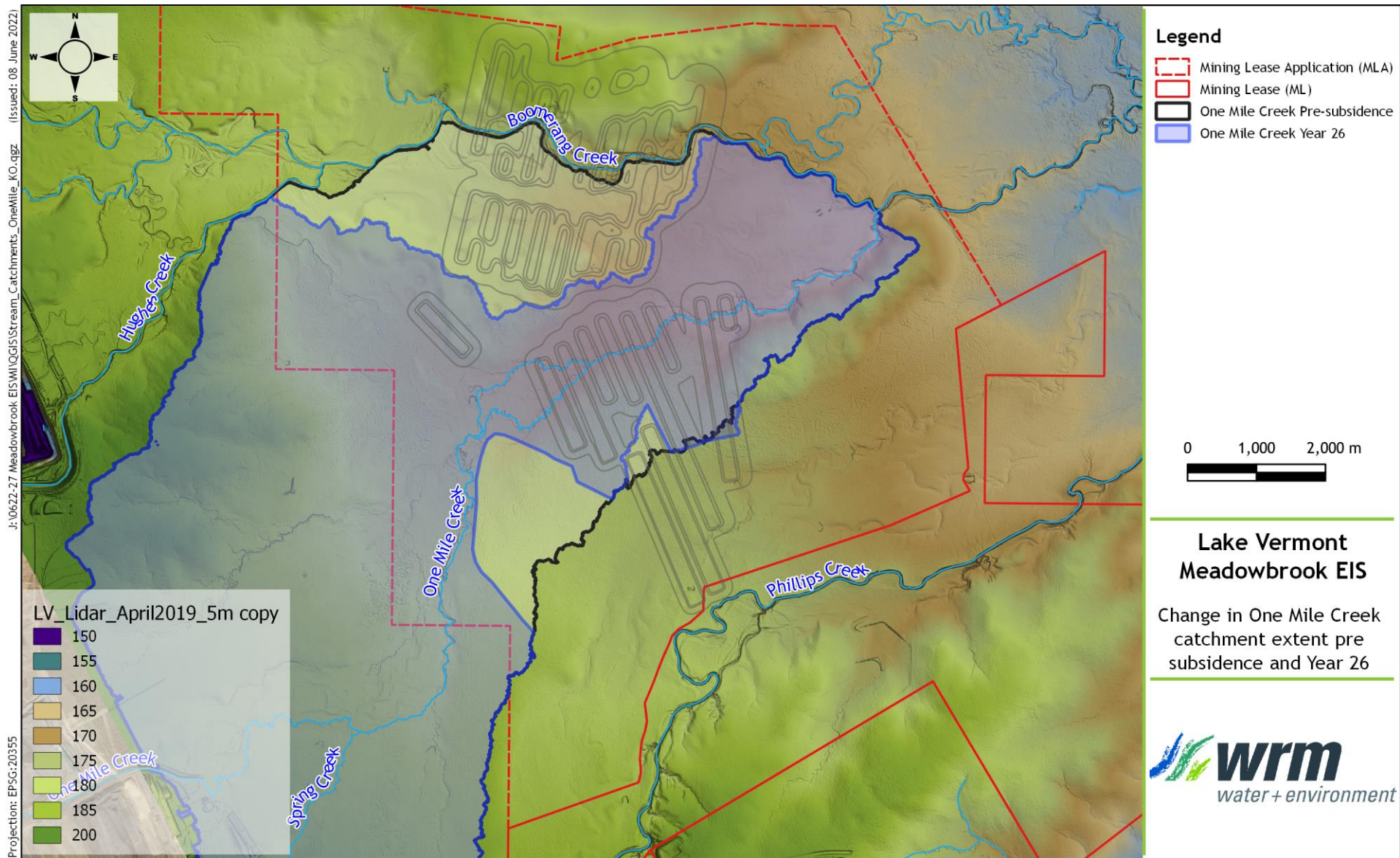
Figure 3.19 - Changes in flow paths - with mitigation works - One Mile Creek - maximum open cut disturbance
