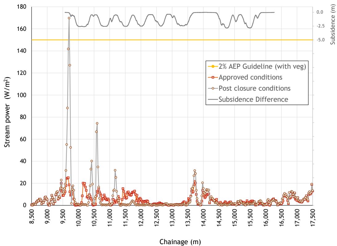
Figure 4.23 - One Mile Creek - 2% AEP - stream power
