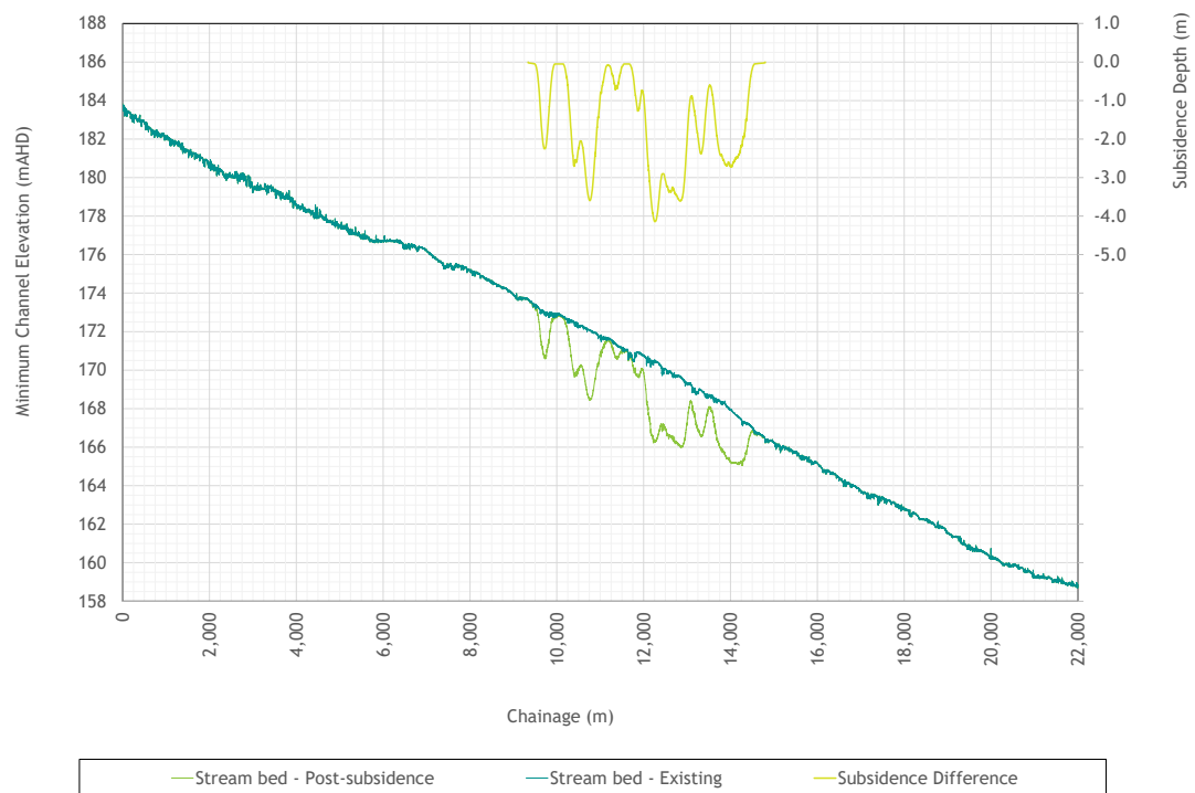
Figure 3.21 - Longitudinal profile Boomerang Creek main channel
