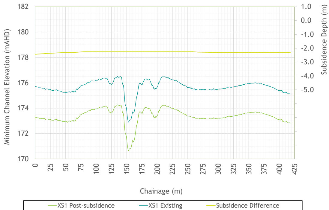
Figure 3.23 - Cross-section - Boomerang Creek main channel Ch 9,720
