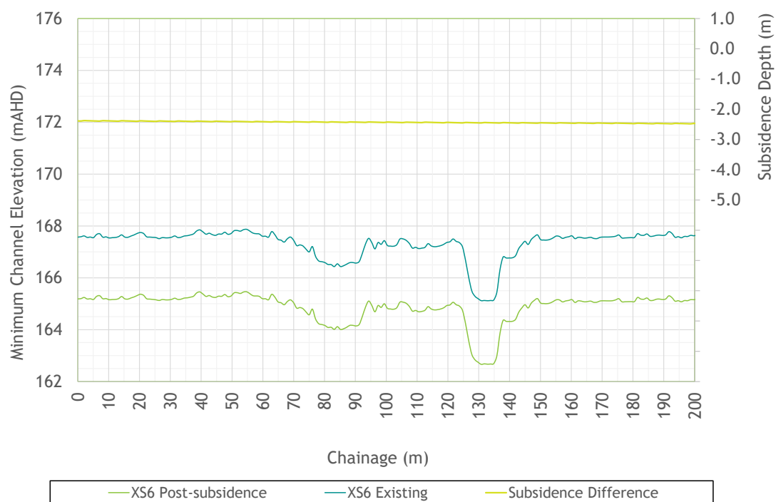
Figure 3.36 - Cross-sections - One Mile Creek main channel Ch 14,690
