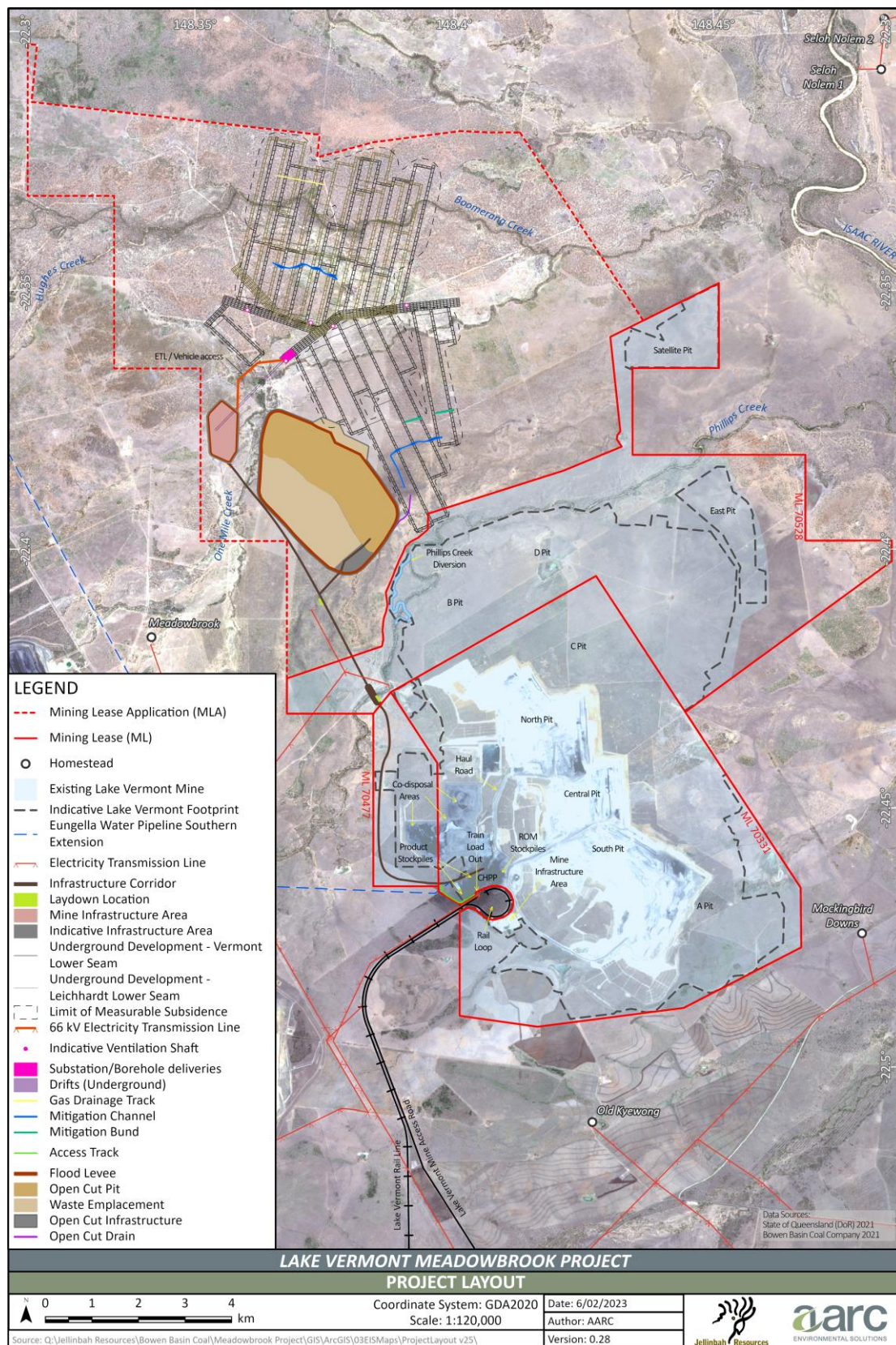
Figure 1.2 - Project layout
