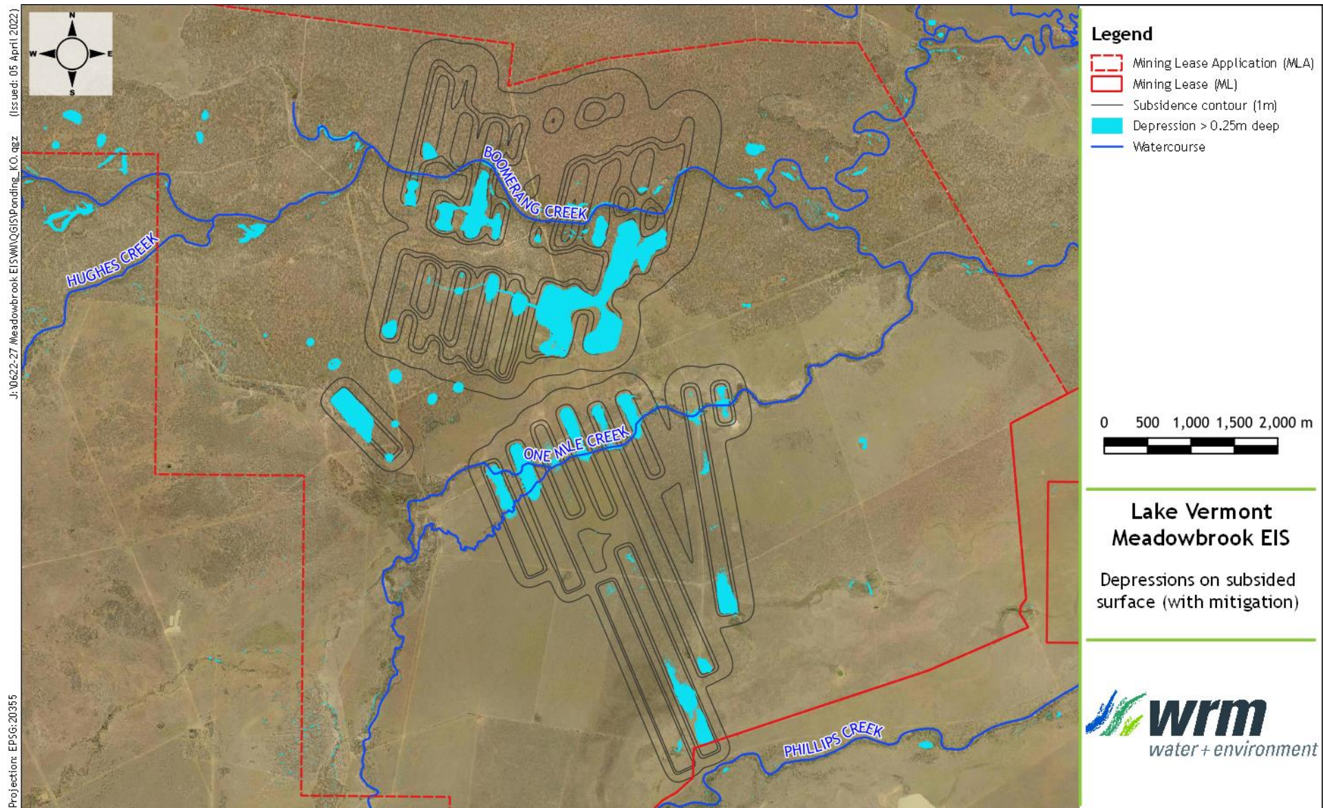
Figure 3.12 - Post-subsidence ponding (mitigated)
