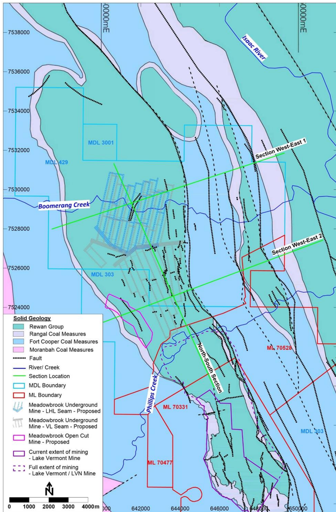
Figure 2.1 - Solid geology
