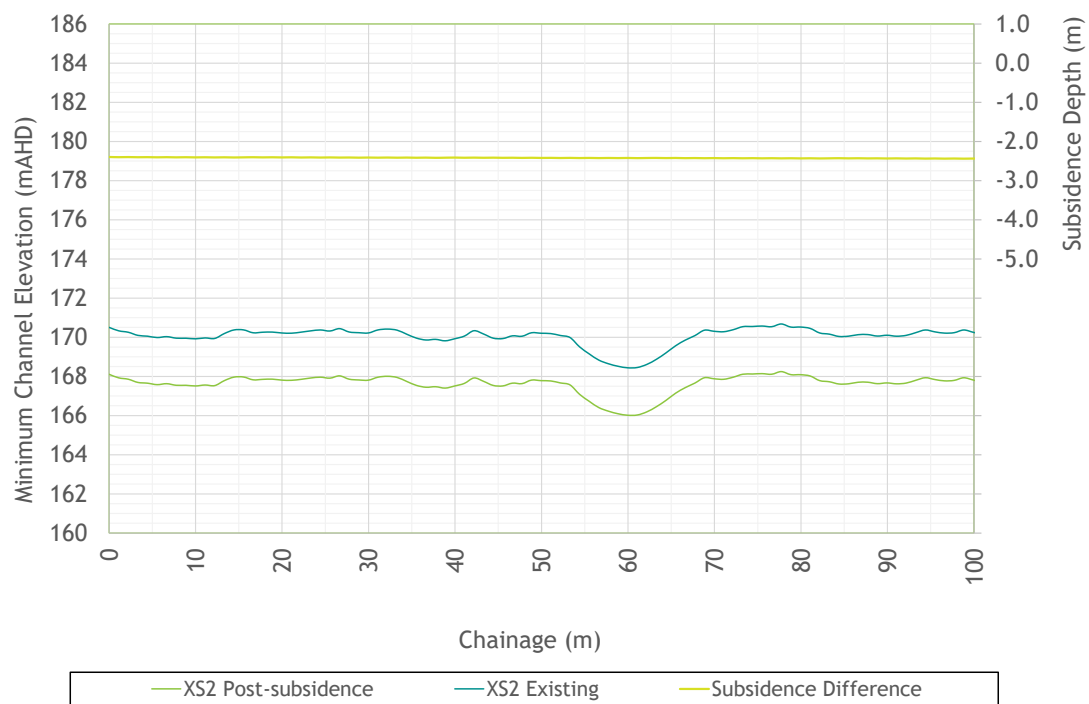
Figure 3.32 - Cross-sections - One Mile Creek main channel Ch 11,440
