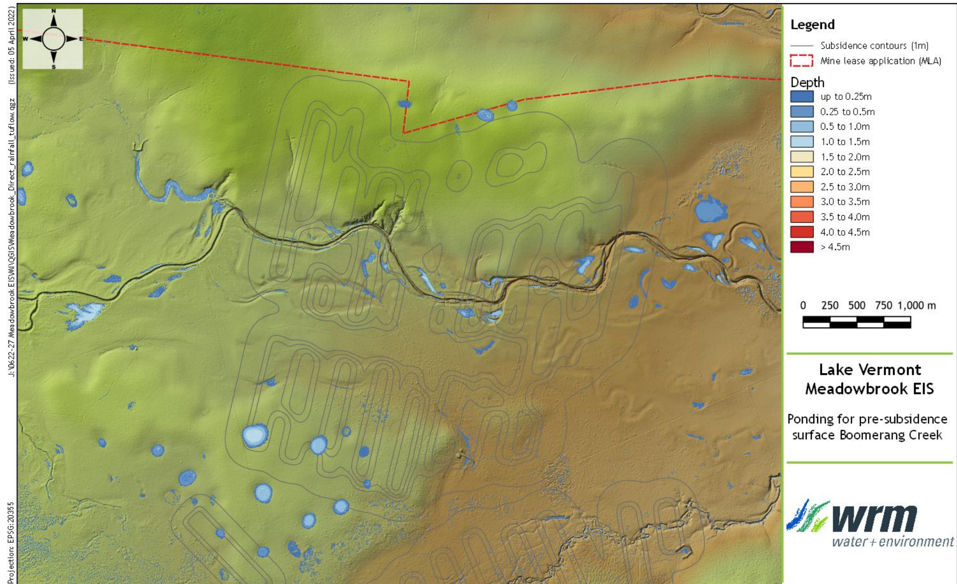
Figure 3.13 - Pre-subsidence ponding (Boomerang Creek)
