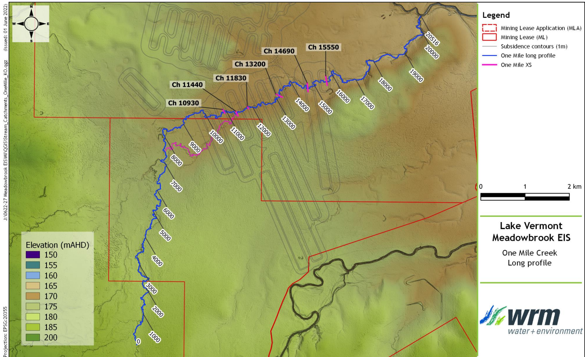
Figure 3.30 - Longitudinal profile chainages - One Mile Creek main channel
