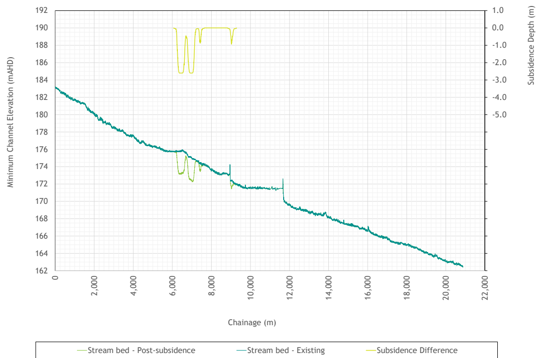
Figure 3.37 - Phillips Creek floodplain
