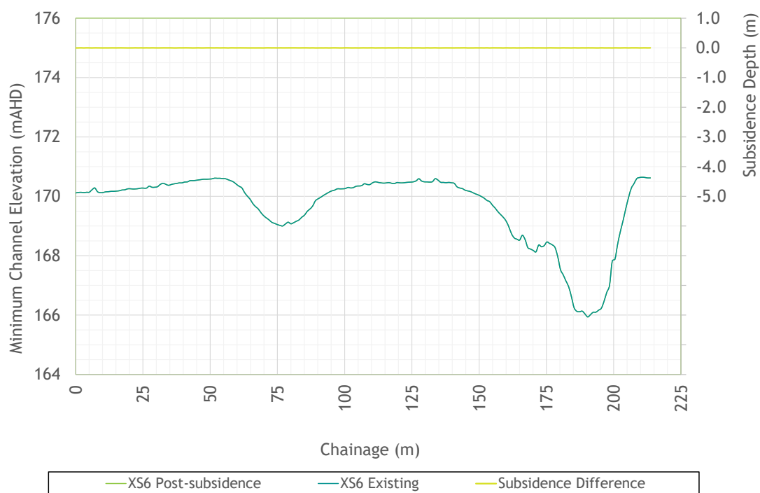
Figure 3.28 - Cross-section - Boomerang Creek main channel Ch 15,190
