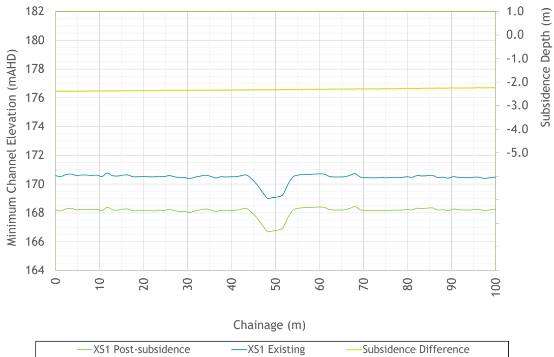
Figure 3.31 - Cross-sections - One Mile Creek main channel Ch 10,930
