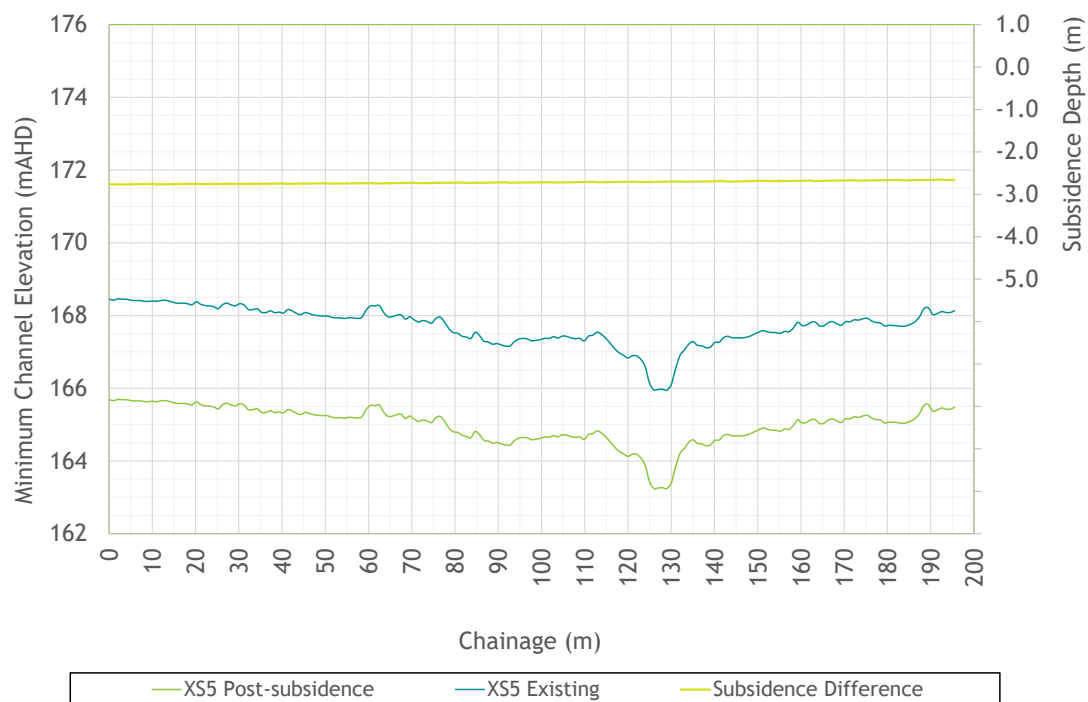
Figure 3.35 - Cross-sections - One Mile Creek main channel Ch 14,690
