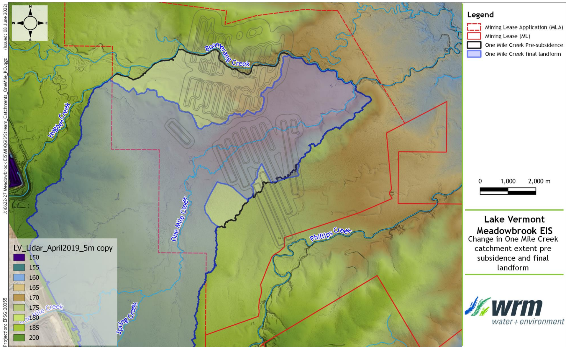
Figure 3.20 - Changes in flow paths - with mitigation works - One Mile Creek - final landform
