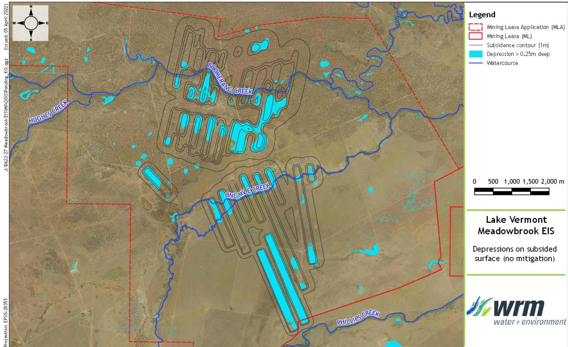
Figure 3.9 - Post-subsidence ponding (unmitigated)
