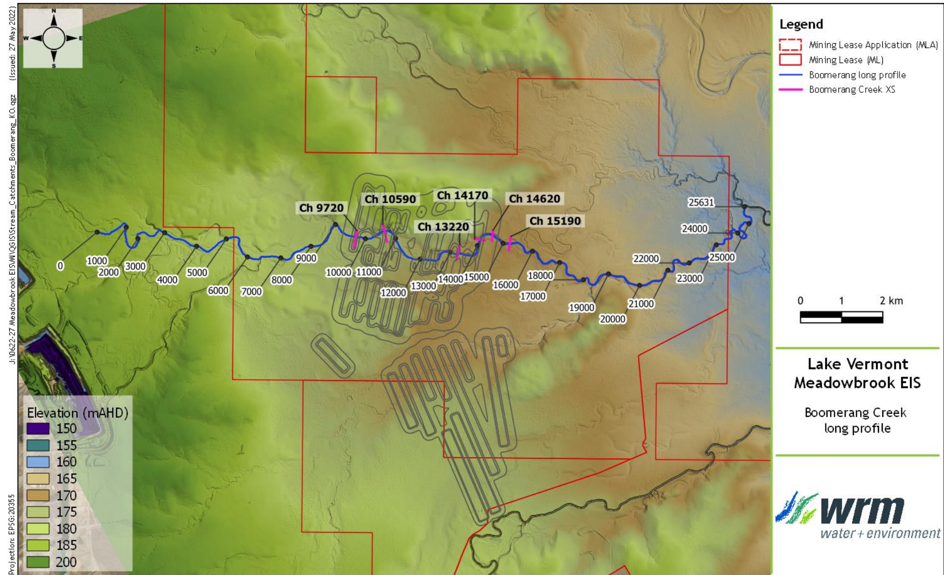
Figure 3.22 - Longitudinal profile chainages and cross-section locations - Boomerang Creek main channel
