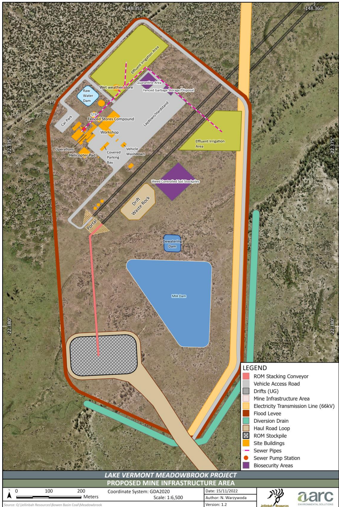
Figure 5.1 - MIA Layout
