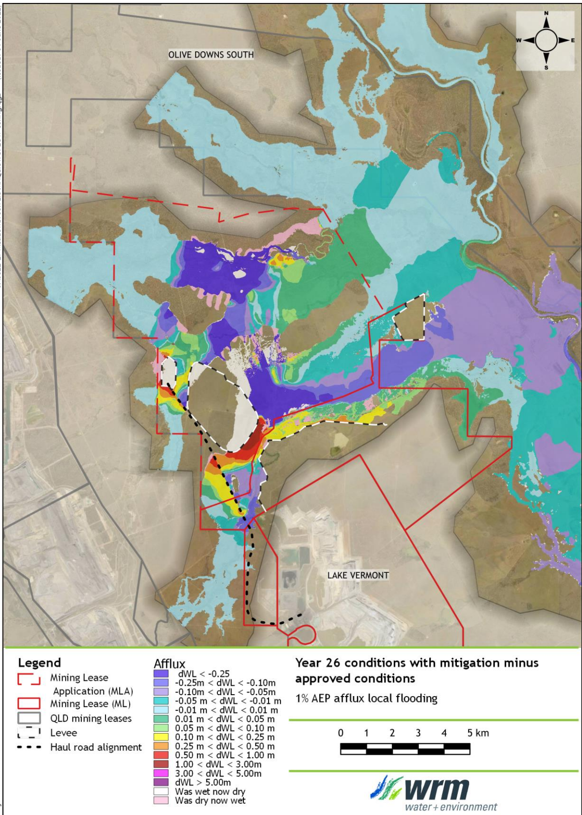
Figure 7.4 - 1% AEP increase in flood depth - Year 26
