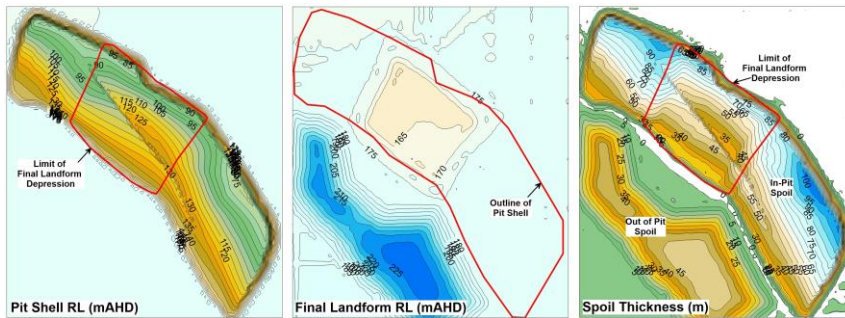
Figure 7.7 - Final landform depression catchments and land use (source: JBT, 2022)
