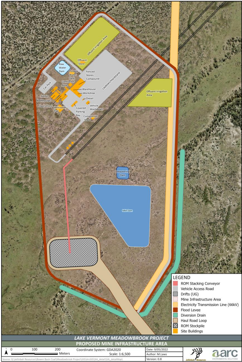
Figure 5.1 - MIA Layout
