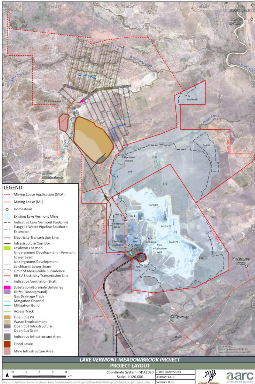
Figure 1.2 - Project layout
