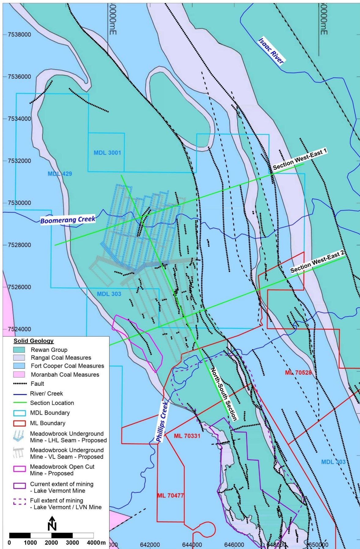
Figure 16: Solid geology of the Project area
