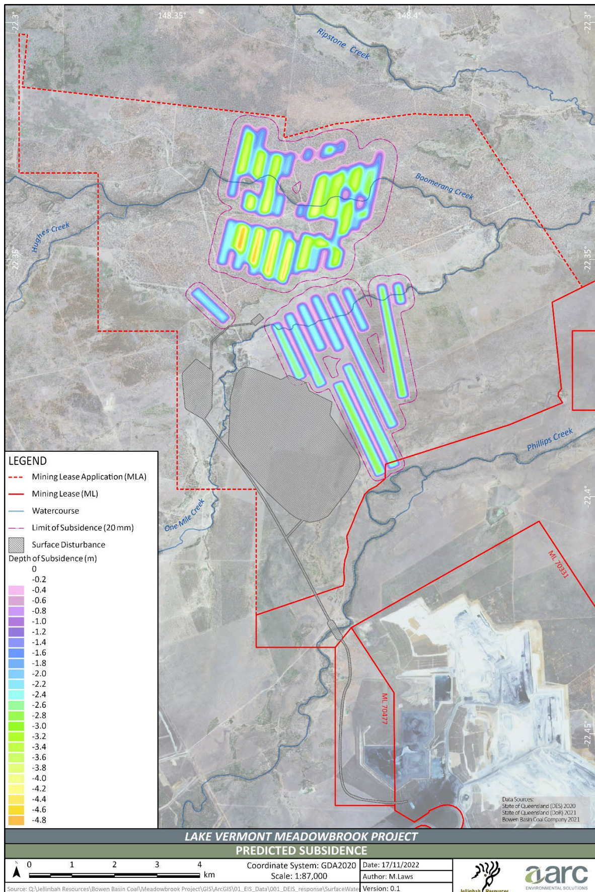
Figure 36: Predicted subsidence after underground mining
