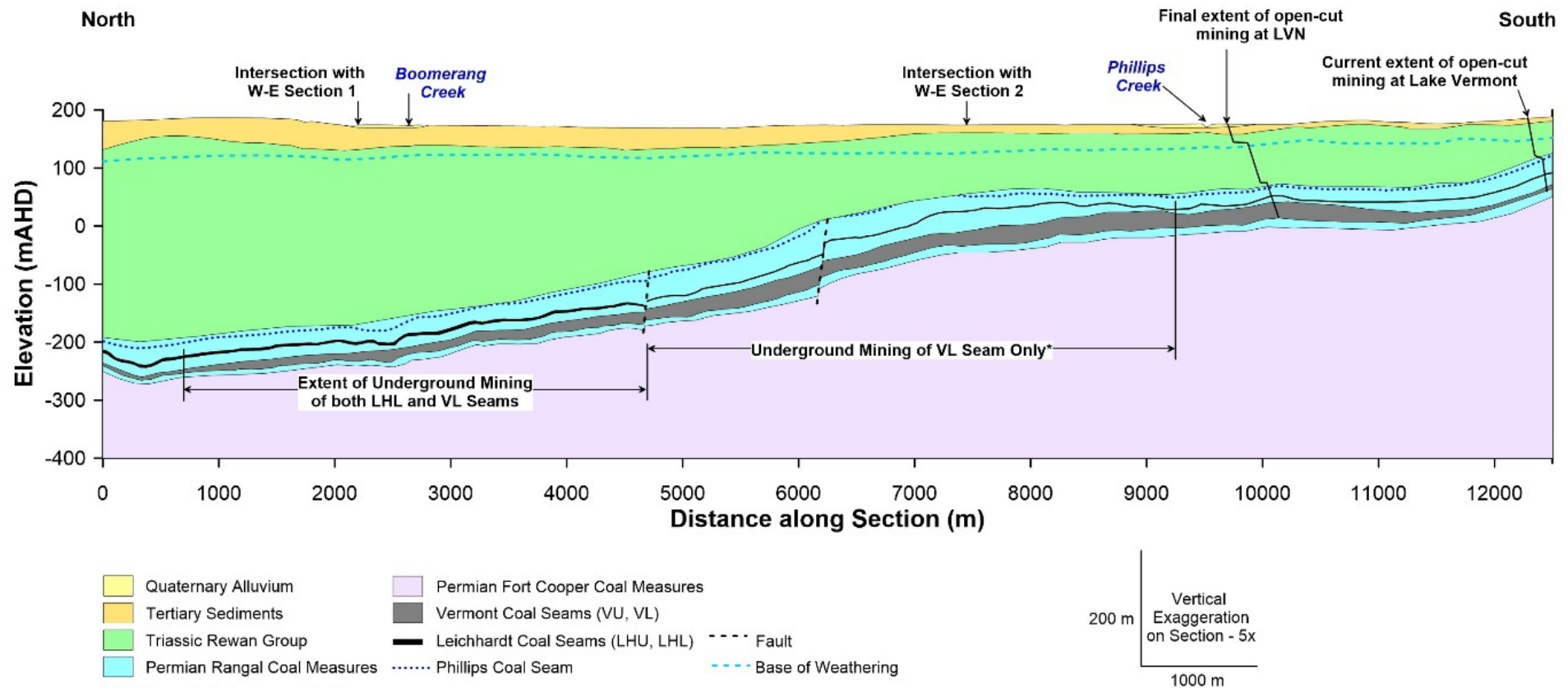
Figure 17: Indicative cross-section of Project geology
