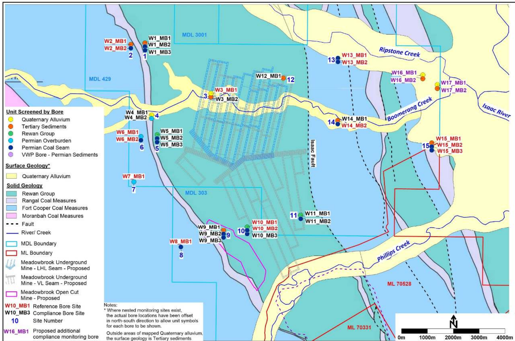
Figure 4-1: Locations of Proposed Compliance and Reference Bores
